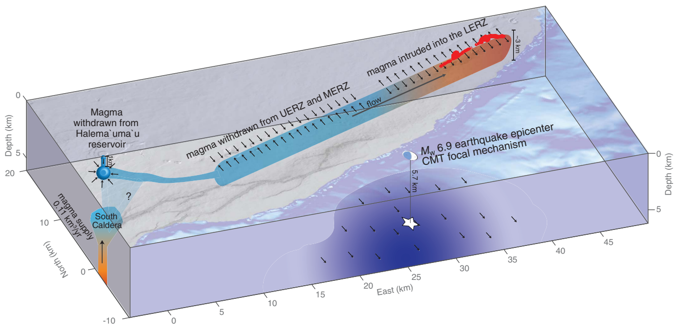
Fig. 6. Schematic representation of the subsurface redistribution of magma during the 2018 Kilauea eruptions. Orange colors depict areas that inflated, whereas turquoise indicates areas from which magma was withdrawn. Dark blue shading shows the approximate extent of the slip model from Fig. 3.
