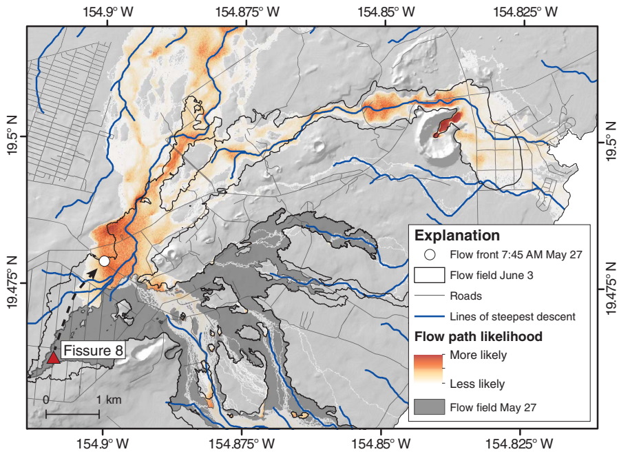
Fig. 4. Example lava flow forecast map. Initial lava flow path forecast for the fissure 8 (red triangle) flow on 27 May (light orange to red colors) compared to the mapped flow extent on 3 June (black outline) and pre-eruptive lines of steepest descent [blue lines; (16)]. Potential flow paths were simulated with DOWNFLOW (17) from approximate flow-front positions reported by field crews (in this case, at the flow margin on the road, rather than from the true inaccessible flow front further east) and pre-eruptive topography updated within the extent of new flows. Resulting maps were preliminary for operational use and produced on-demand as the flows progressed, following decades of syn-eruptive flow mapping and expanding the past use of steepest-descent paths for flow modeling. The dashed arrow indicates the approximate initial flow from which the flow-front emanates.
