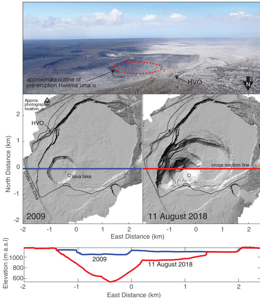
Fig. 5. Digital elevation changes at the summit of Kilauea Volcano. LIDAR (light detection and ranging) digital elevation models (DEMs) of Kilauea's summit from 2009 (left) and 11 August 2018 (right), showing the collapse of the caldera. Black lines indicate roads; the locations of the HVO and former lava lake are indicated. The red and blue lines correspond to the locations of the cross sections shown at the bottom. The difference between the 2009 and 2018 topographic profiles gives the amount of subsidence that occurred almost entirely since 1 May 2018. The photo at the top was taken northwest of the caldera looking to the southeast after the collapse. a.s.l., above sea level.
