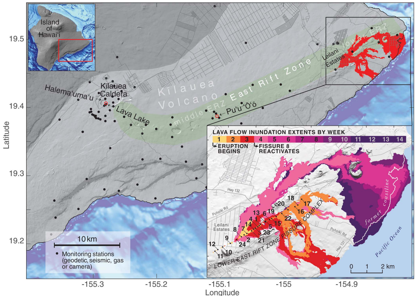
Fig. 1. Map showing the location of Kīlauea Volcano on the island of Hawai'i and the general geographic features of the volcano. Kīlauea Volcano is indicated in light gray. Gray lines are roads, and dots mark the locations of monitoring stations (geodetic, seismic, gas, or camera). Locations of summit and Pu'u 'Ō'ō eruptive vents are indicated with red
