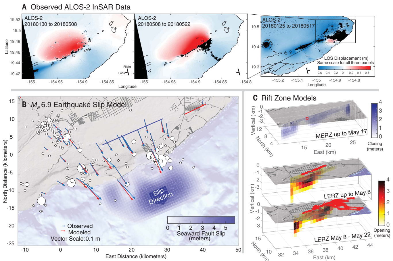
Fig. 3. Surface deformation and models of 2018 eruptive and earthquake activity. (A) Example InSAR line-of-sight (LOS) displacement data from the ALOS-2 satellite used during the eruption (scale bar is the same for all three images). (B) GNSS displacements and model of the 4 May M_w 6.9 earthquake (vector uncertainties are smaller than the arrowheads). White circles are earthquakes. (C) Example models
